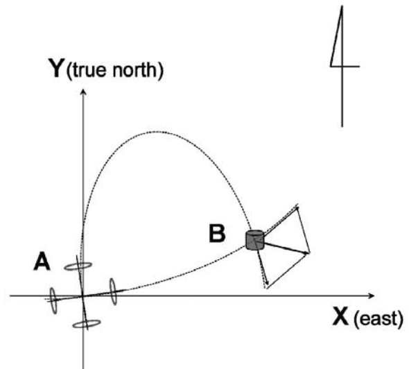
Figure 3 Schematic diagram of declination angle measurement
